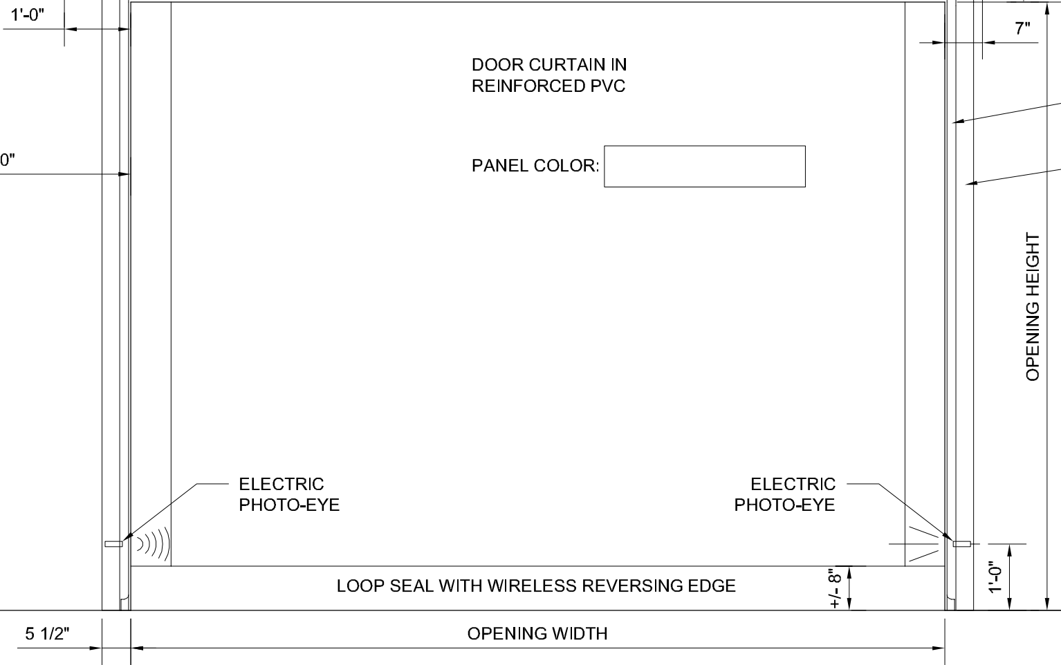
ELEVATION VIEW - FRONT
