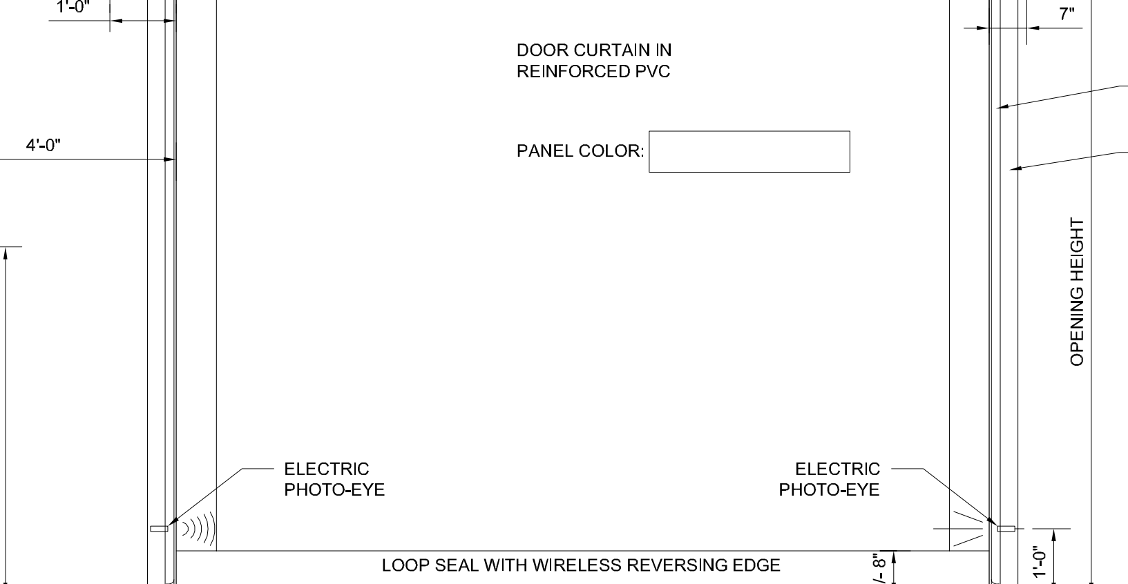
ELEVATION VIEW - FRONT
