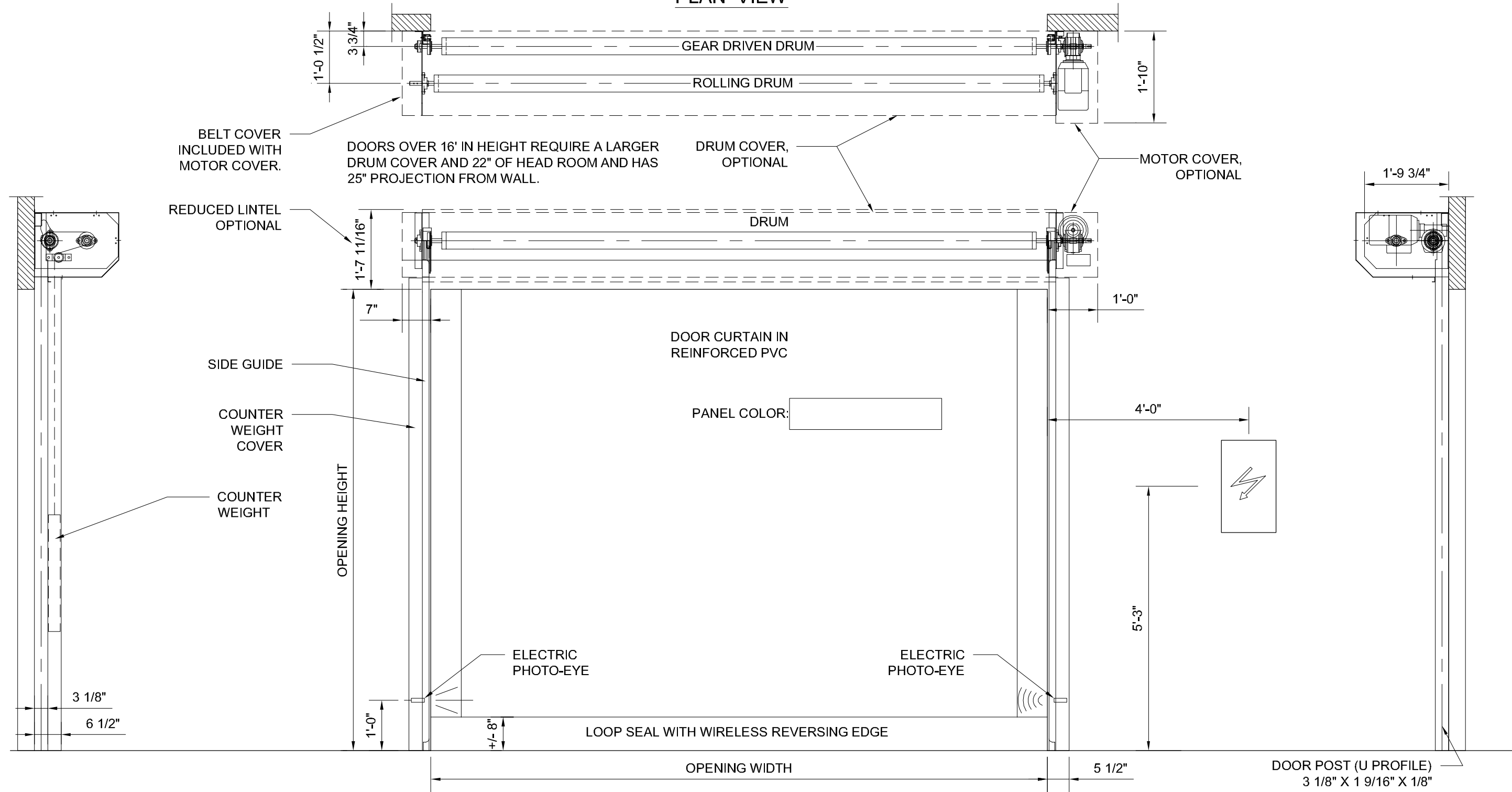
ELEVATION VIEW - LEFT
